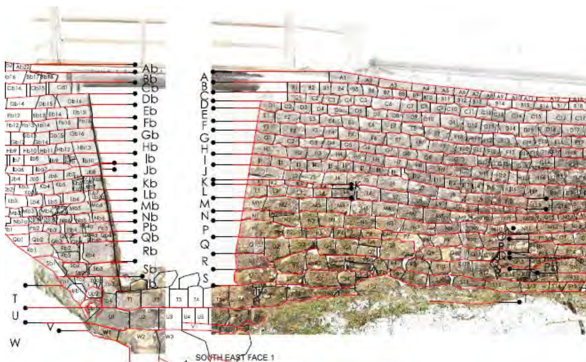
Figure 2-10: Excerpt of section showing individually recorded stones. (Delaney Civil, 2023)
