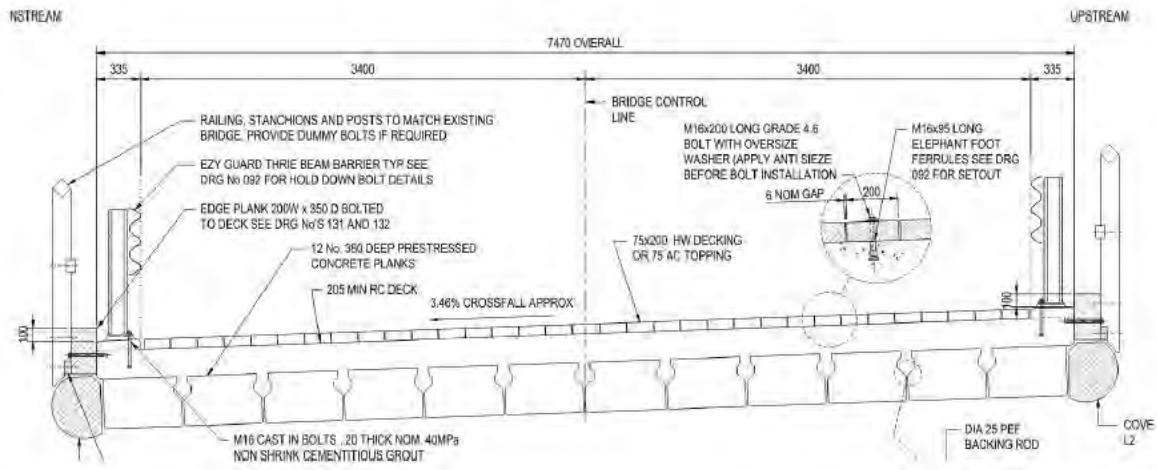
Figure 2-13: Excerpt of structure cross section of bridge reconstruction design. Source: Turnbull, 2023.
