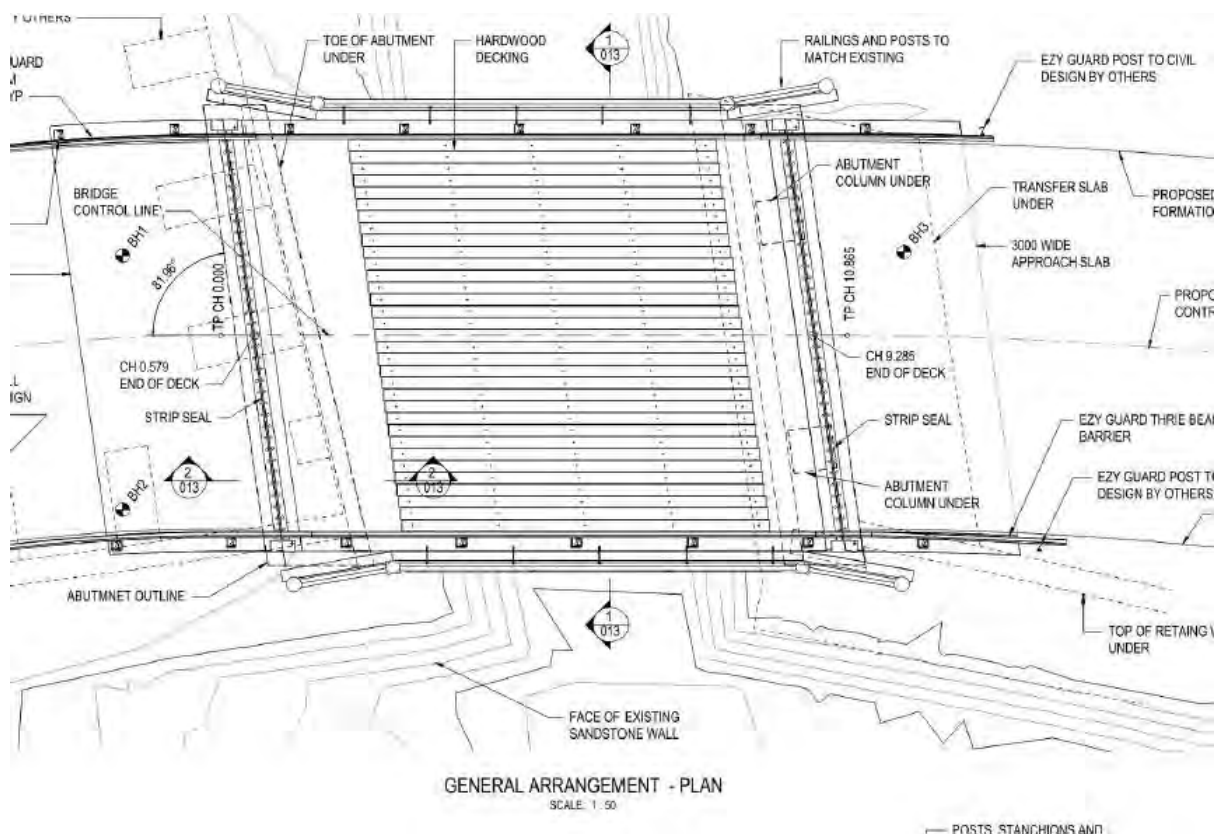
Figure 2-12: Excerpt of plan of bridge reconstruction design. Source: Turnbull, 2023.
