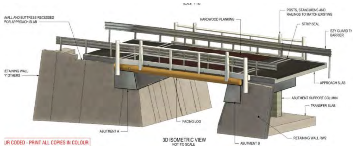
Figure 2-11: Excerpt of isometric 3D depiction of new bridge design (note, not showing stone reinstatement), showing deck reinstatement, timber balustrade reinstatement, and additional new conforming barrier. Source: Turnbull, 2023.
