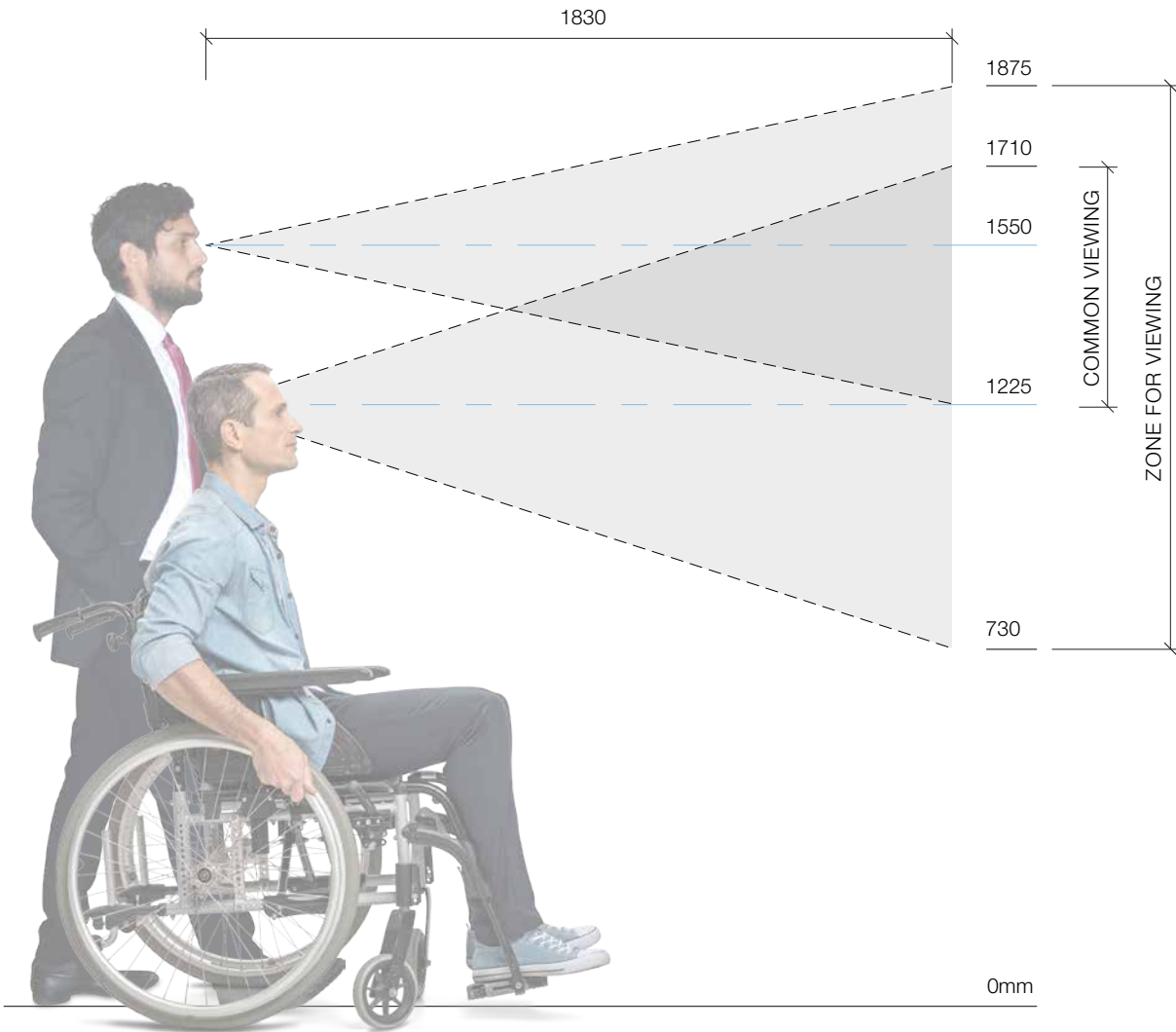
Legible viewing distances required for signage
