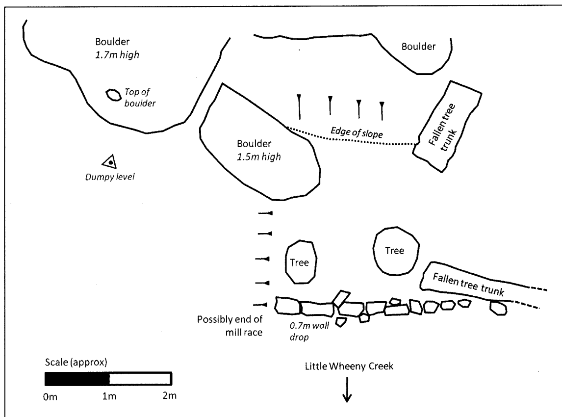
Figure 2. Plan of the Dam Area (10/10/09)
