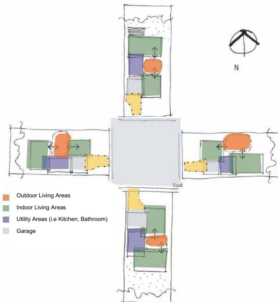
Figure 4.17 Dwelling Layouts for Solar Access
