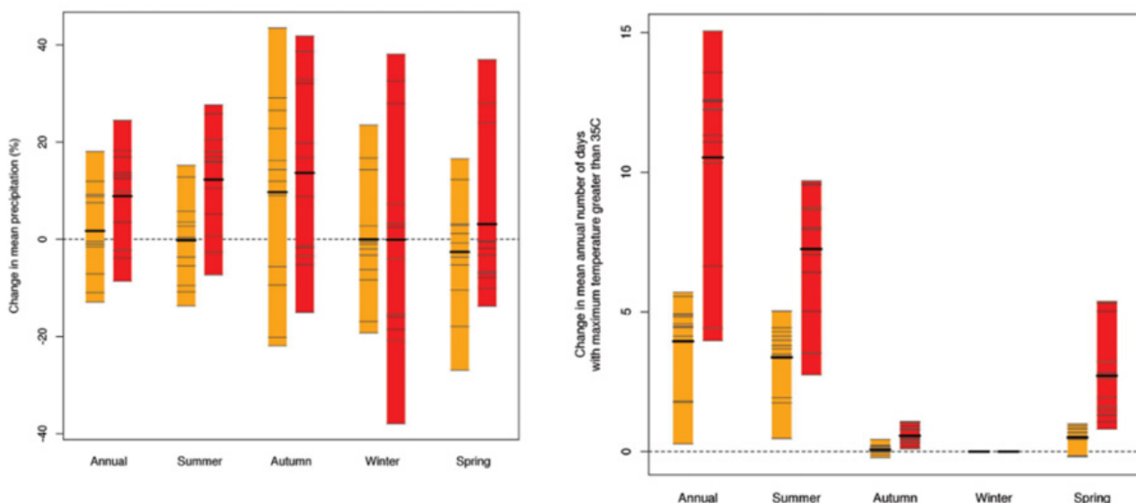
Figure 8: Projected annual and seasonal change in the number of hot days (with daily maximum temperature > 35°C ) for the Sydney metropolitan region from the NARCLIM 1.0 project (Source: OEH, 2014).
