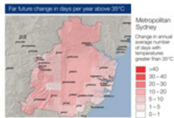
Figure 9: Far future (2060–2078) projected changes in the number of days per year with maximum temperatures above 35°C.
