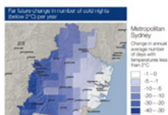
Figure 12: Far future (2060–2078) projected changes in the number of nights per year with minimum temperatures below 2°C, compared to the baseline period (1990–2008).
